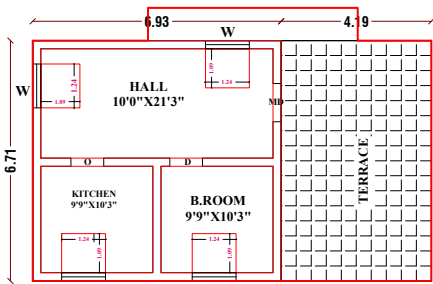
PRO.FIRST FLOOR PLAN
