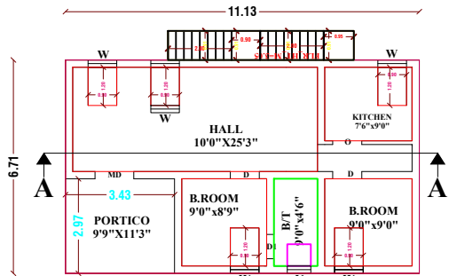
EXI.GROUND FLOOR PLAN
