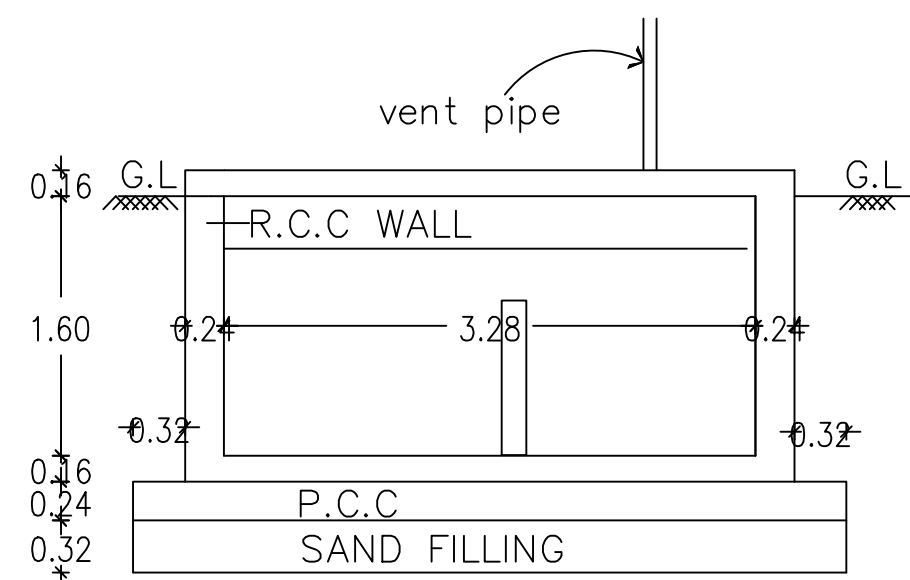
SECTION OF SEPTICK ON D-D
