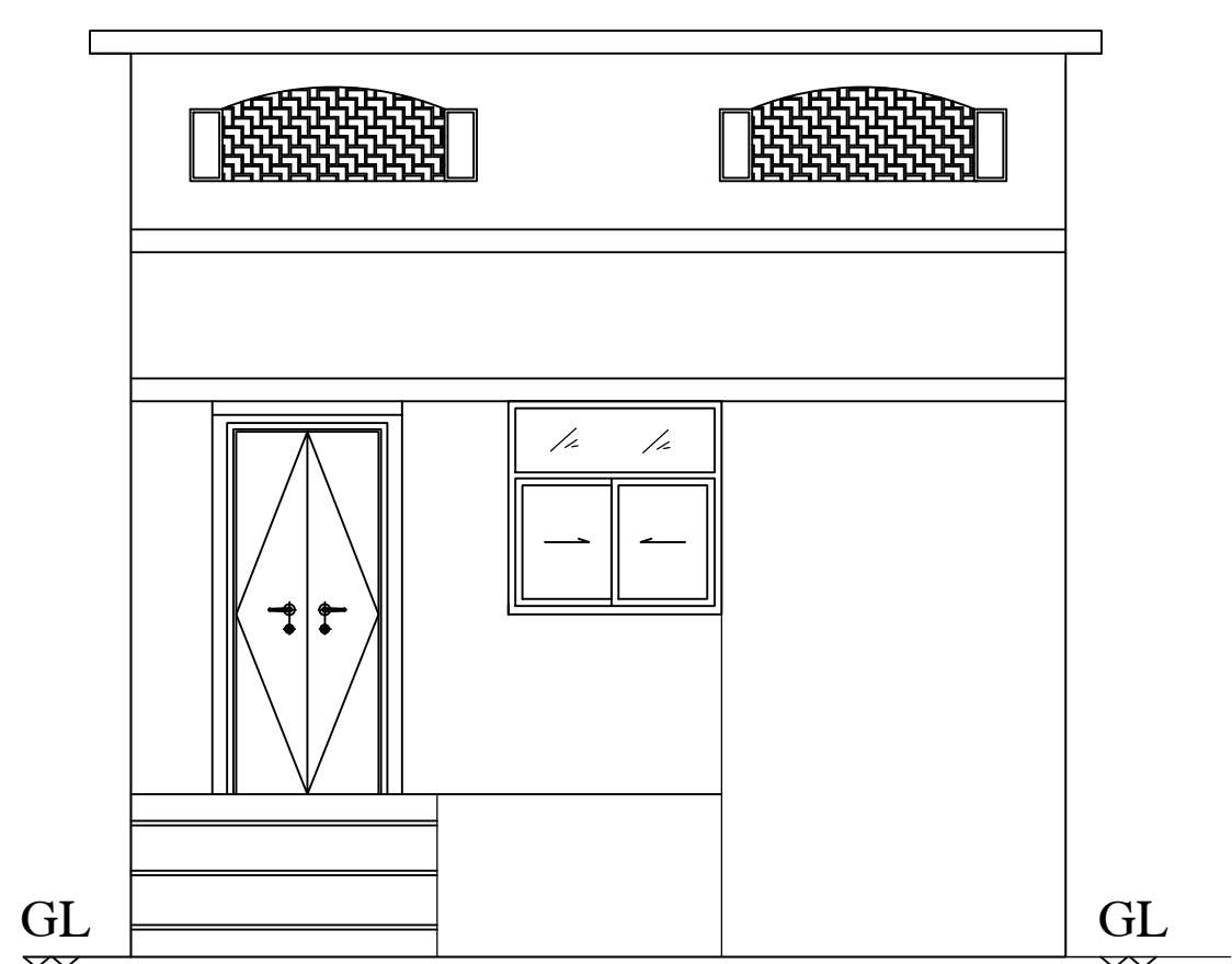
FRONT ELEVATION
