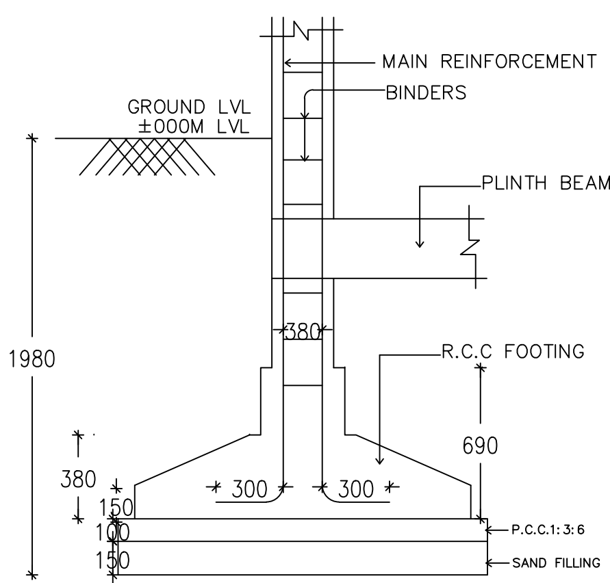
TYPICAL SECTION OF R.C.C COLUMN FOUNDATION
