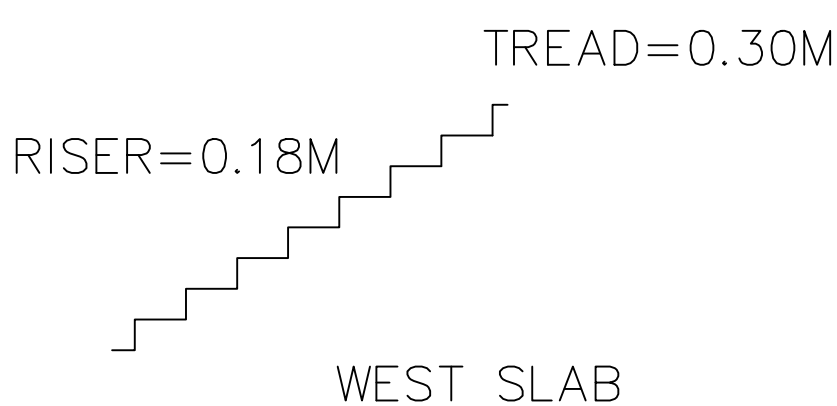
STAIR CASE DETAILS
