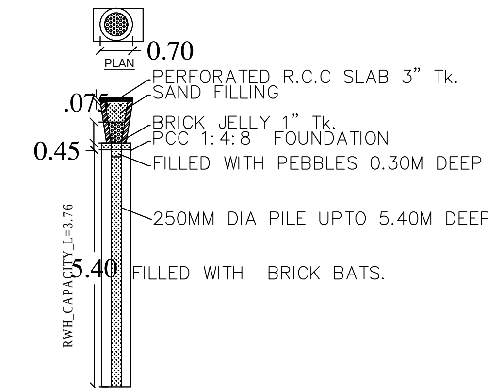
PERCOLATION PIT SECTION OF RAIN WATER
