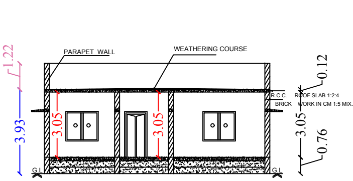
Section on-"AA"
