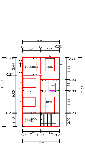
PLAN
