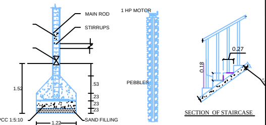
BORE WELL
