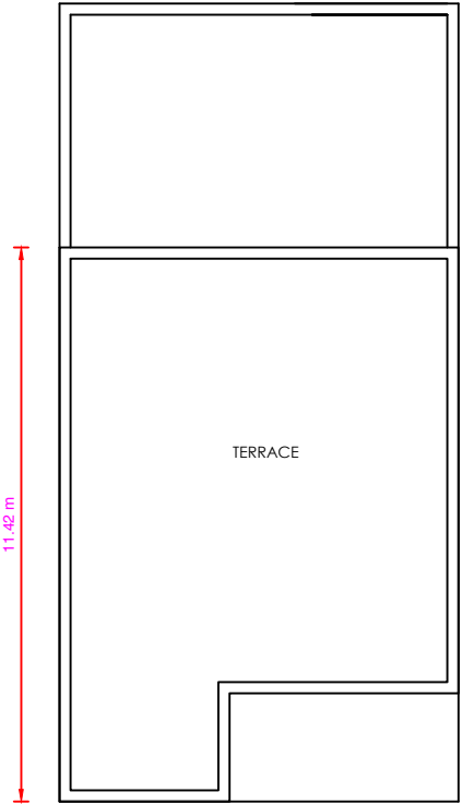
TERRACE FLOOR
