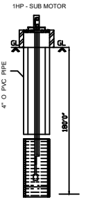
Bore Well Details
