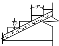
STAIR CASE DETAILS
