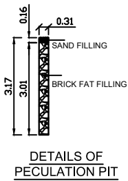
DETAILS OF PECULATION PIT
