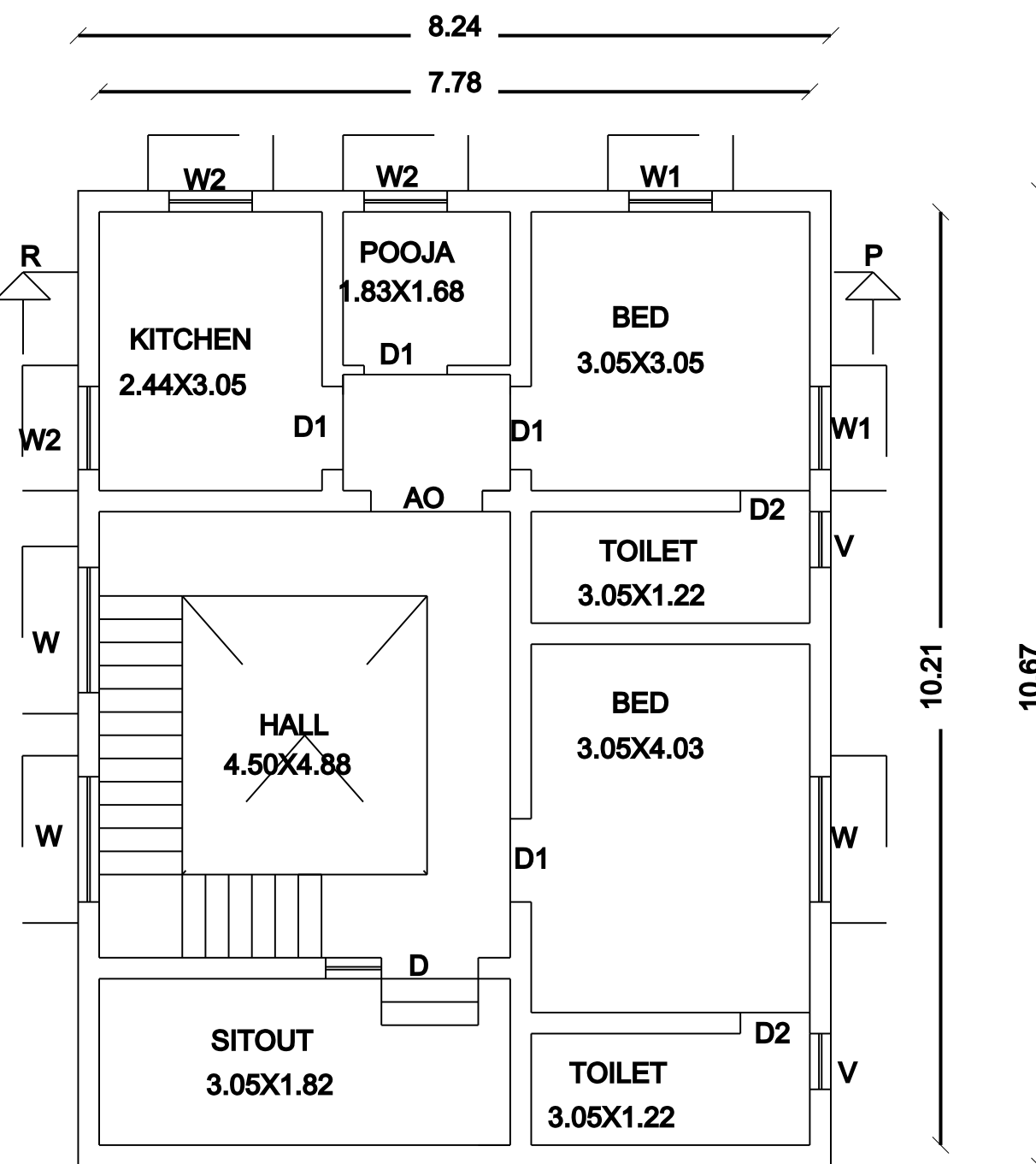
EX-GROUND FLOOR PLAN
