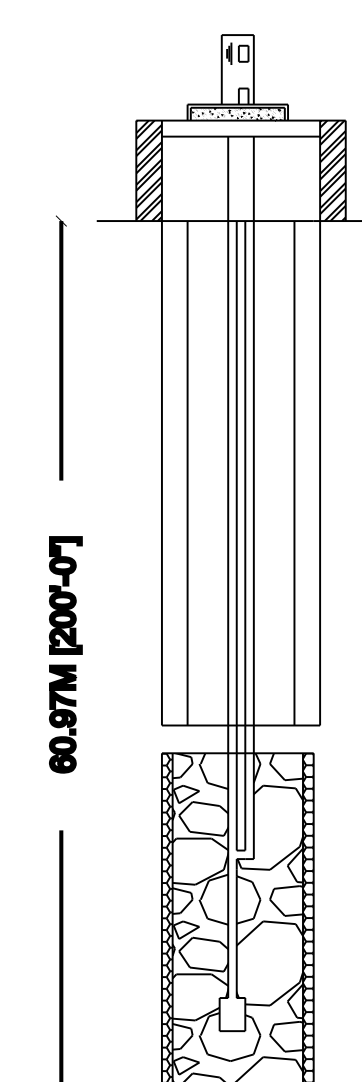
BORE WELL DETAILS
