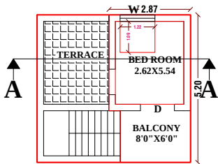
PRO.FIRST FLOOR PLAN
