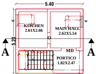
EXI.GROUND FLOOR PLAN
