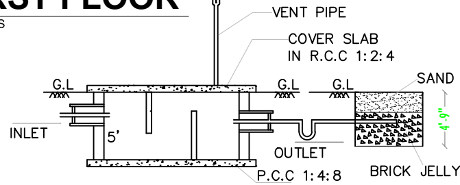
SECTION-AB
