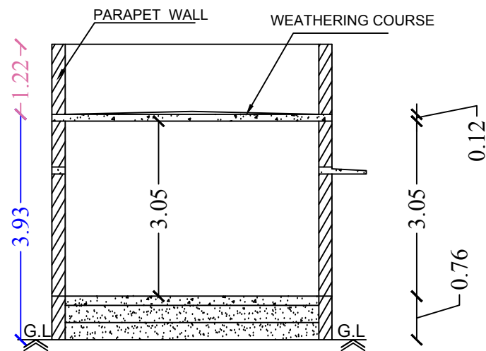
Section on-"AA"
