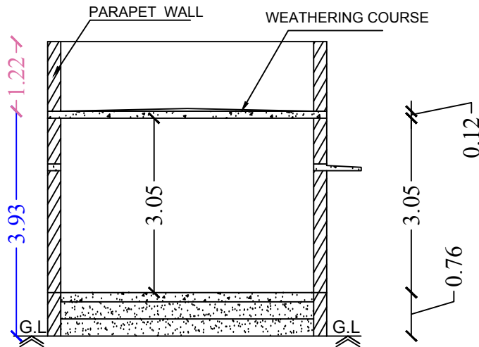
Section on-"AA"
