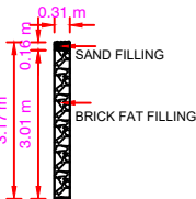
DETAILS OF PECCULATION PIT
