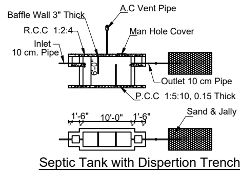
Septic Tank with Dispersion Trench
