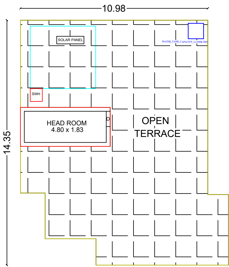
HEAD ROOM & TERRACE FLOOR PLAN
