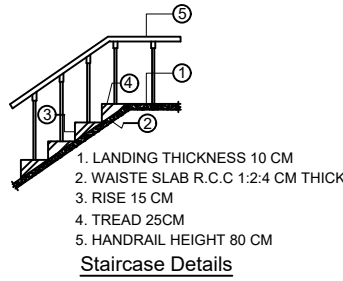
Staircase Details
