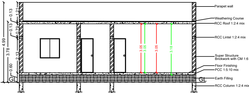
SECTION ON "VR"
