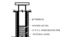
BOREWELL DETAILS
