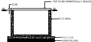
SECTION ON BB SCALE 1:100
