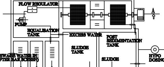
SEWAGE TREATMENT PLANT DETAILS WASTEWATER RECYCLING UNIT
