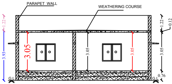
Section on-"AA"
