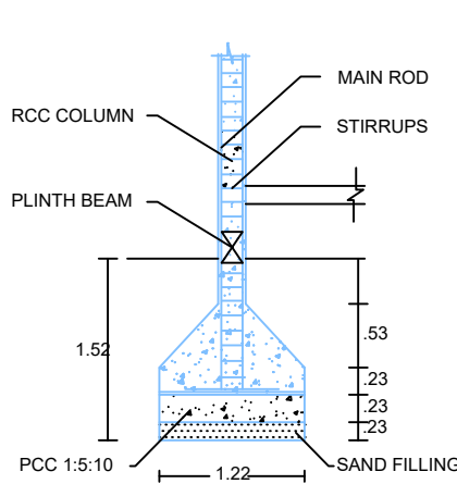
COLUMN DETAILS
