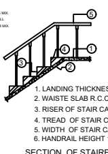
SECTION OF STAIR CASE
