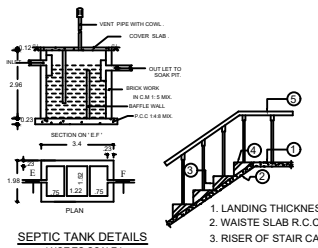
SEPTIC TANK DETAILS (NOT TO SCALE)
