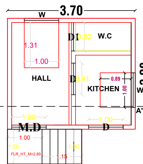
PRO SECOND FLOOR
