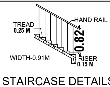
STAIRCASE DETAILS
