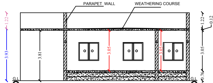
Section on-"AA"
