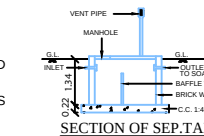
SECTION OF SEP.TANK
