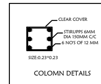
COLOMN DETAILS
