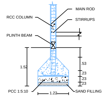
RCC COLUMN PLINTH BEAM
