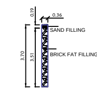
DETAILS OF PERCULATION PIT
