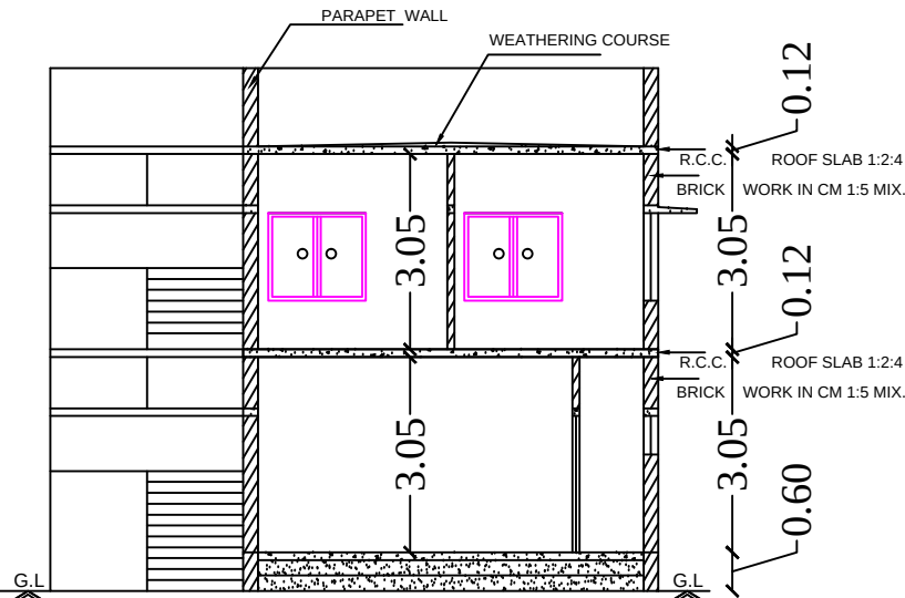
Section on-"AA"
