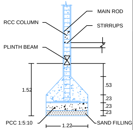
COLUMN DETAILS
