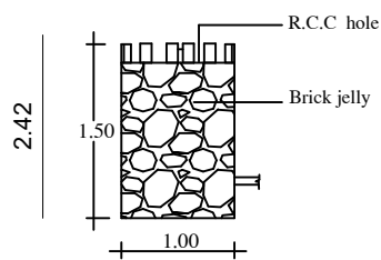
COLLECTING RAIN WATER PIT Not to Scale RWHP_CAPACITY_L=1000 LTRS
