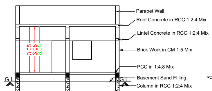
Section RR
