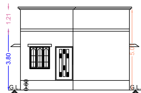
Front Elevation
