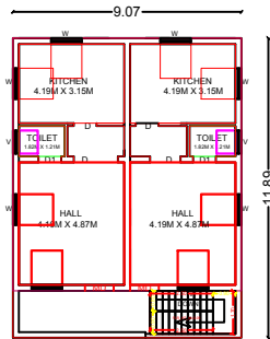
PRO.FIRST FLOOR PLAN
