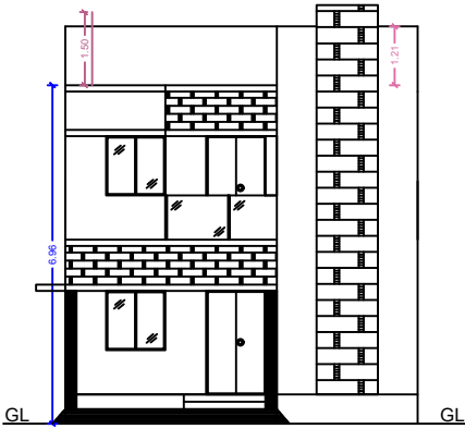
FRONT ELEVATION
