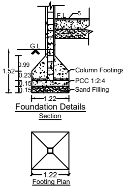
Foundation Details
