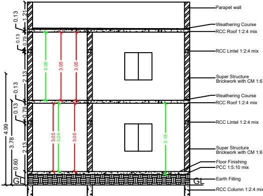
SECTION ON "VR"
