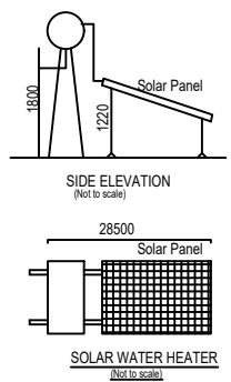
SOLAR WATER HEATER (Not to scale)
