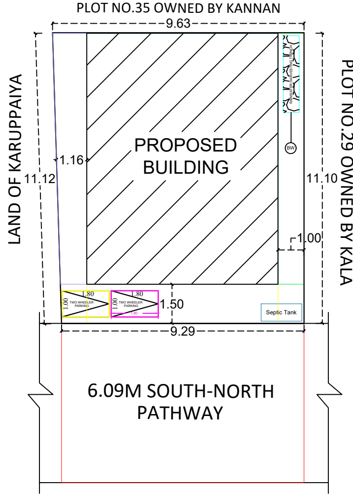
SITE PLAN (1:100)
