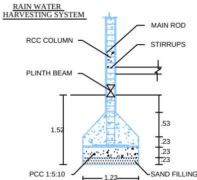
COLUMN DETAILS
