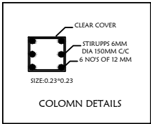
COLUMN DETAILS
