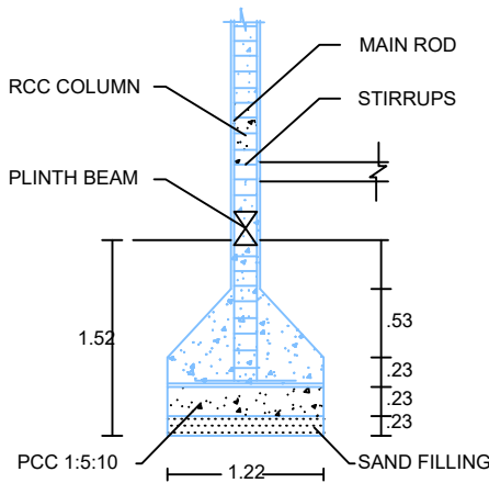
COLUMN DETAILS
