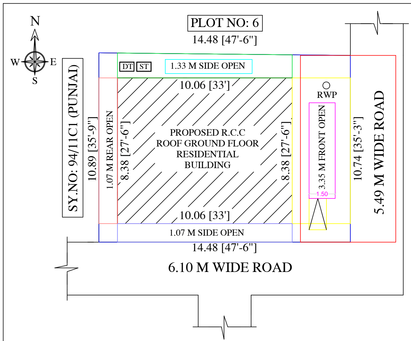
SITE PLAN
