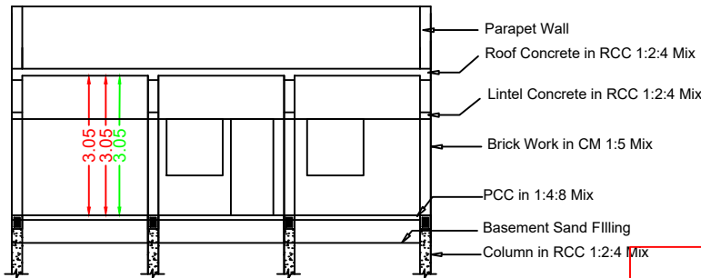
Section RR
