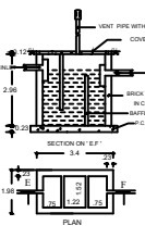
SEPTIC TANK DETAILS (NOT TO SCALE)
