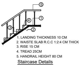
Staircase Details
