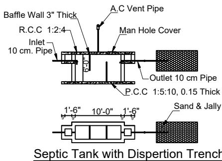
Septic Tank with Dispersion Trench
