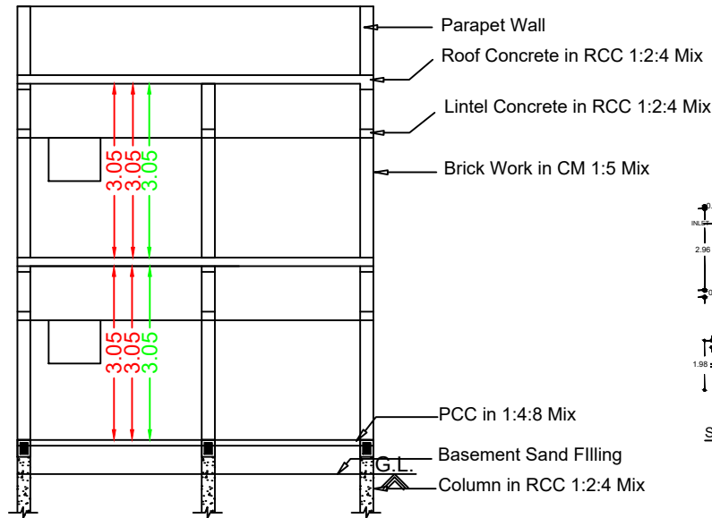
Section RR
