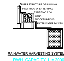
Section RR
