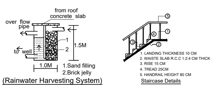
(Rainwater Harvesting System)
