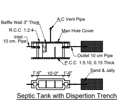
Septic Tank with Dispersion Trench
