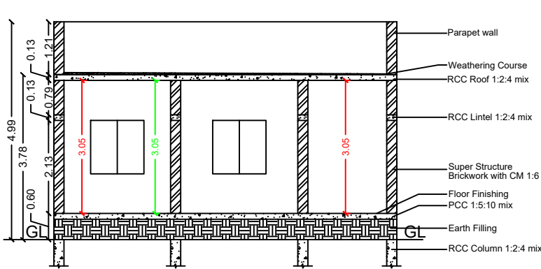
SECTION ON "VR"
