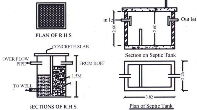
SECTIONS OF R.H.S.
