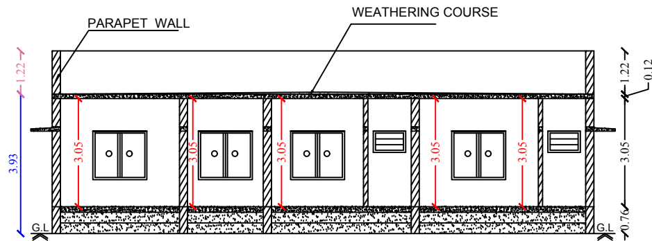
Section on-"AA"
