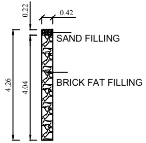
DETAILS OF PERCULATION PIT
