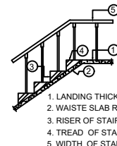
SECTION OF STAIR CASE
