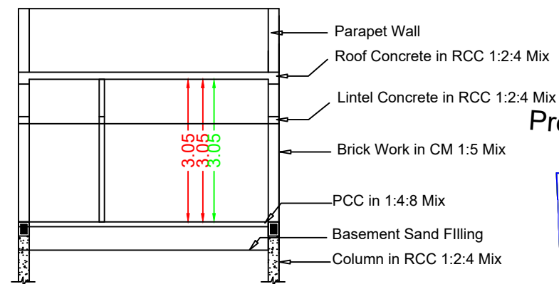
Section RR
