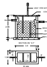
SEPTIC TANK DETAILS ( NOT TO SCALE )
