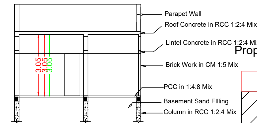
Section RR
