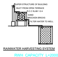
Section RR
