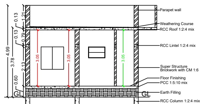
SECTION ON "VR"
