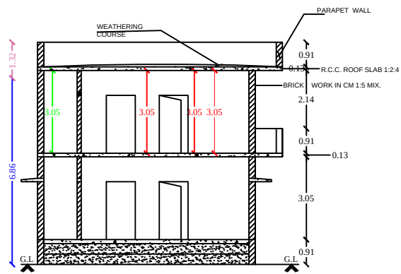
Section on-"AA"
