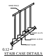
STAIR CASE DETAILS
