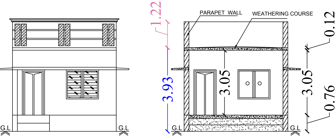
Front Elevation
