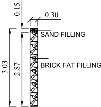
DETAILS OF PERCULATION PIT
