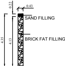
DETAILS OF PERCOLATION PIT
