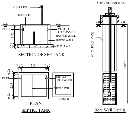
SEPTIC TANK
