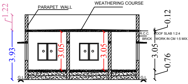
Section on-"AA"
