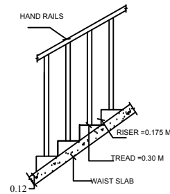
STAIR CASE DETAILS
