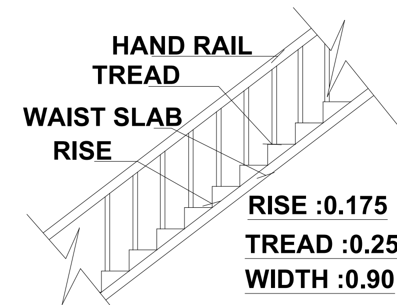
STAIRCASE DETAILS
