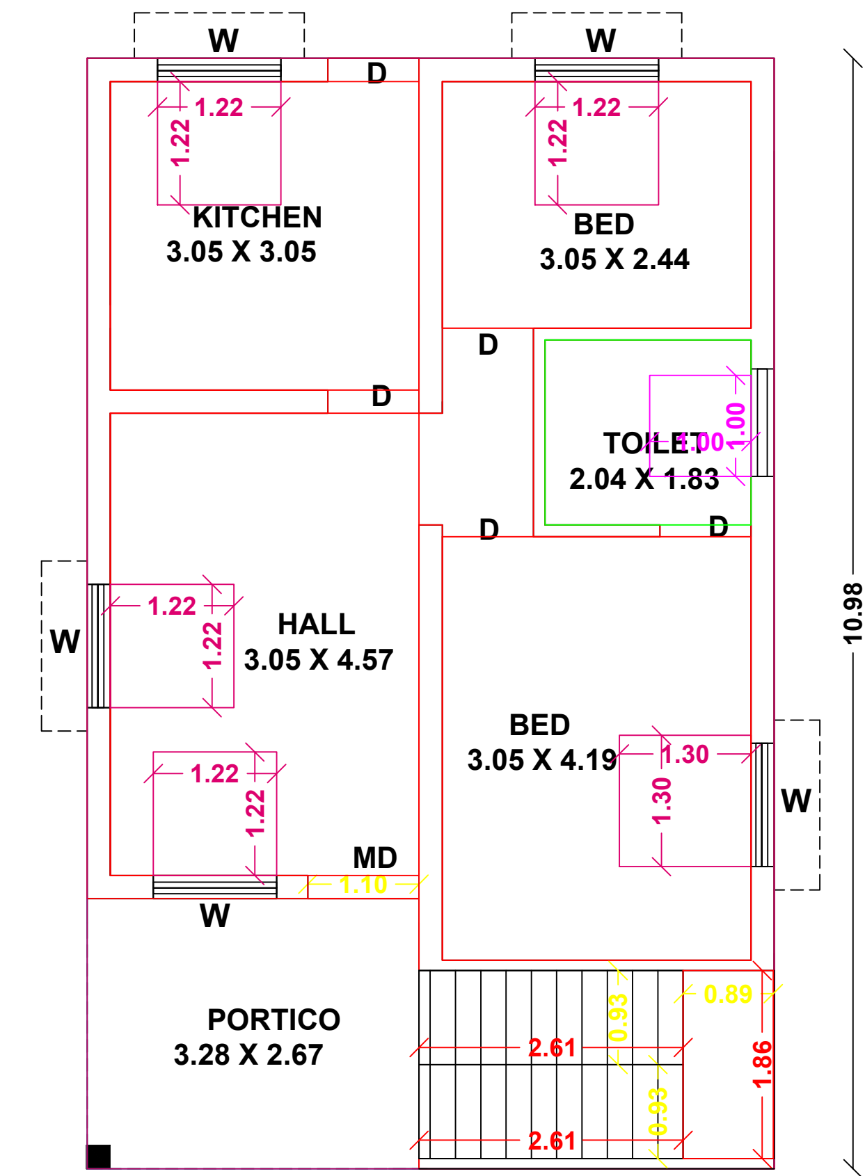
FLOOR-GROUND
