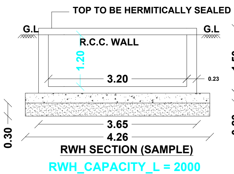
RWV SECTION (SAMPLE)
