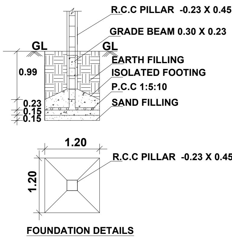
FOUNDATION DETAILS
