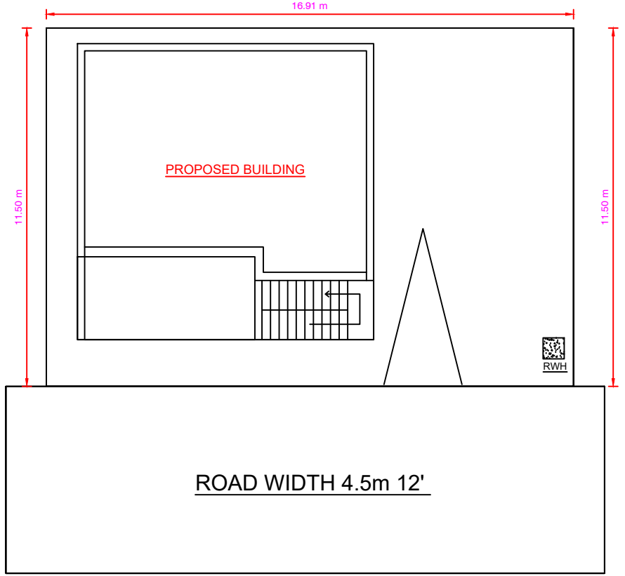
SITE PLAN
