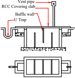
SEPTIC TANK
