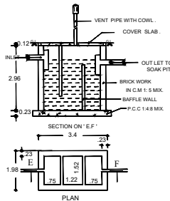
SEPTIC TANK DETAILS (NOT TO SCALE)
