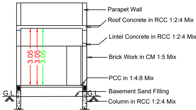
Section RR
