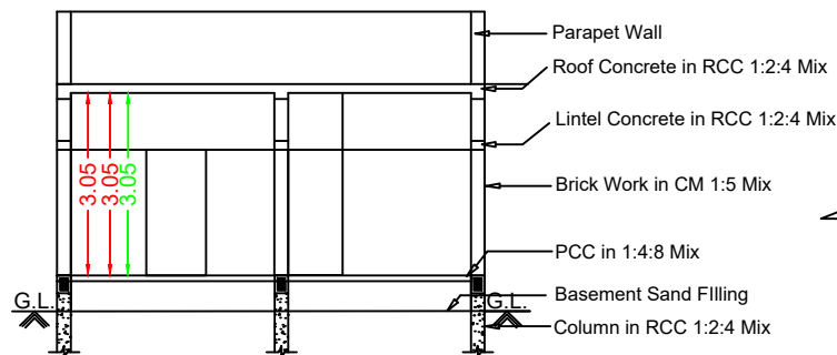
Section RR
