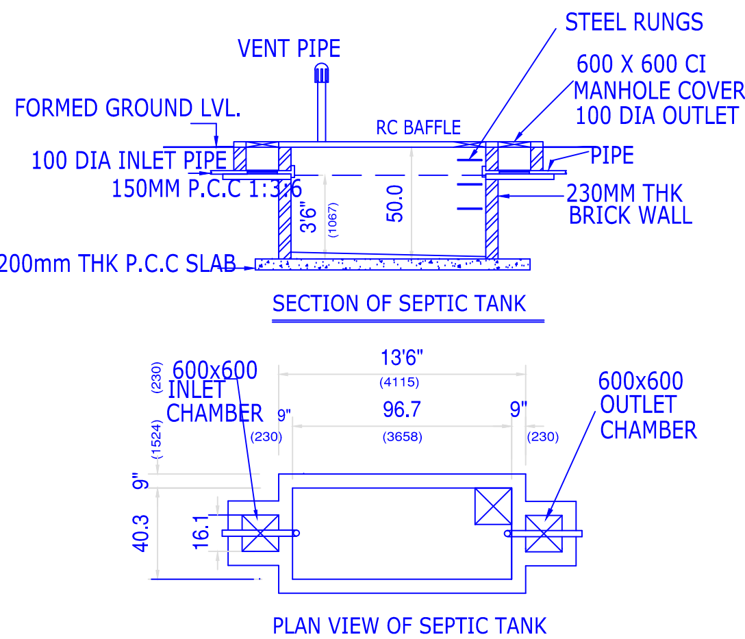
SECTION OF SEPTIC TANK
