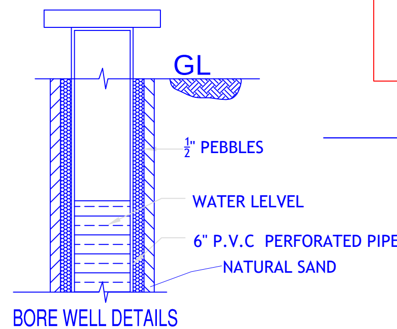
BORE WELL DETAILS
