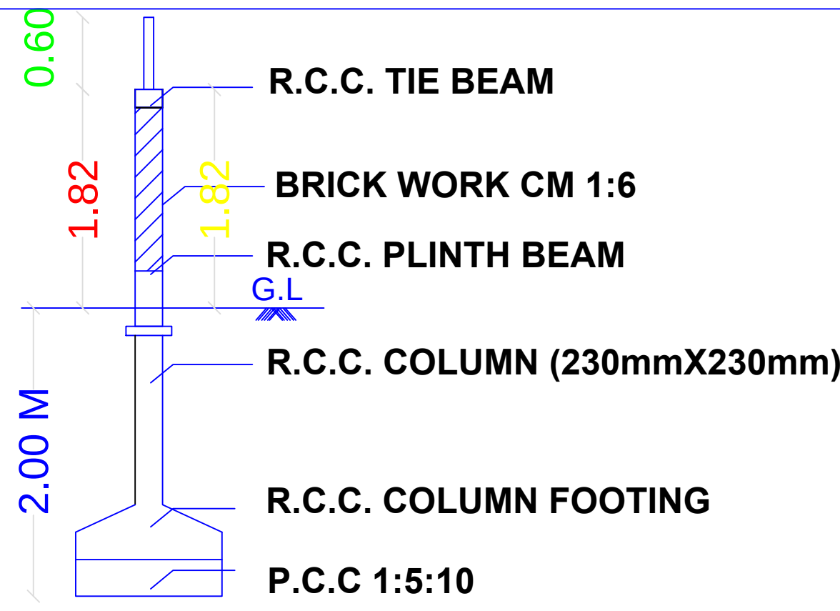
COMPOUND WALL DETAILS
