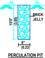
PERCULATION PIT
