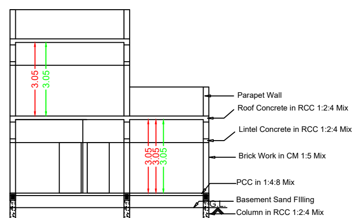
Section RR
