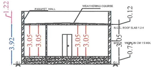
Section on-"AA"
