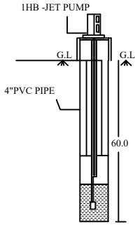
BORE WELL DETAILS
