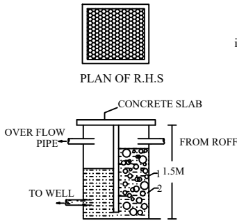
SECTIONS OF R.H.S.
