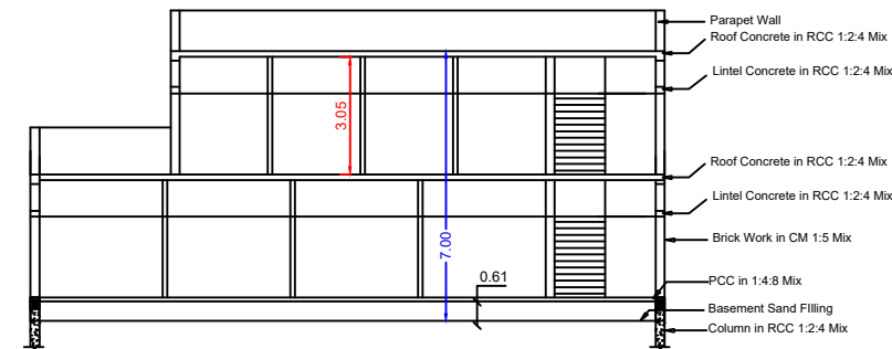
Section RR
